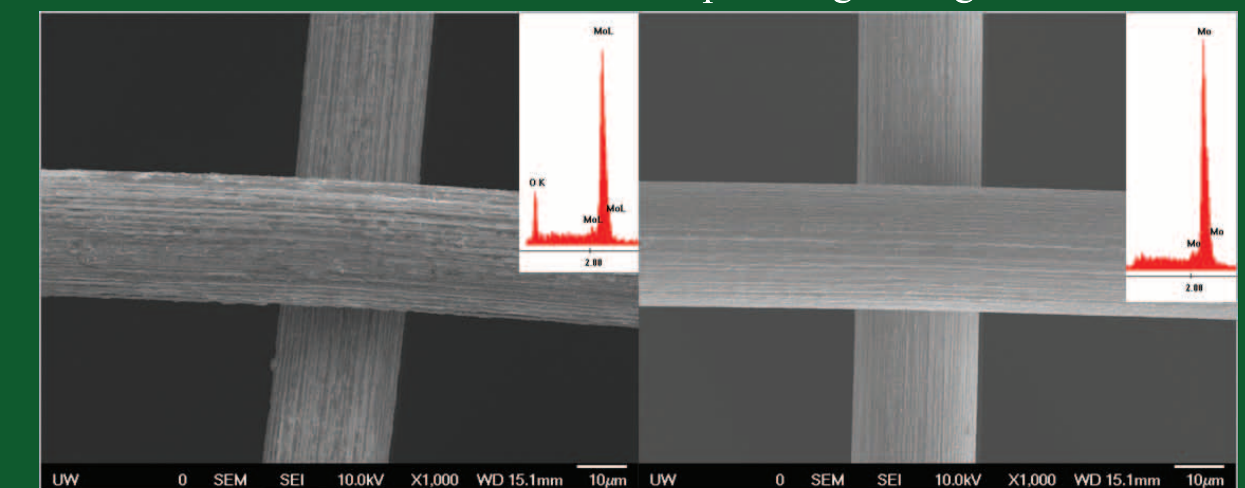
SPG outer molybdenum grid before (Left) and after (Right) 1000 pulses of operation.
