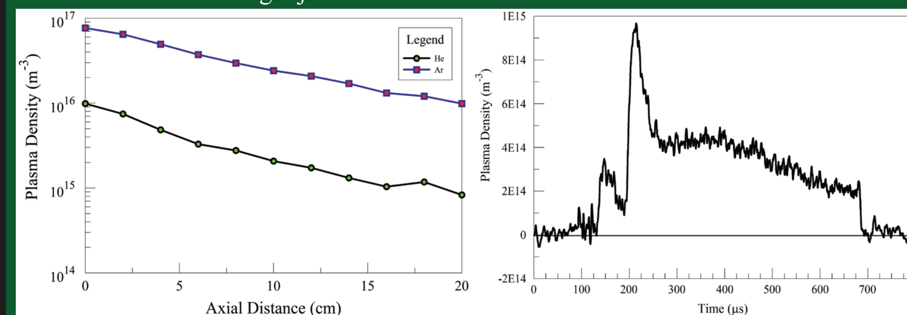
Left: Helium and argon plasma density in the large vacuum chamber as a function of distance downstream from the EPS. Right: Density temporal profile in hydrogen. The plasma is present for 500 \mu s.
