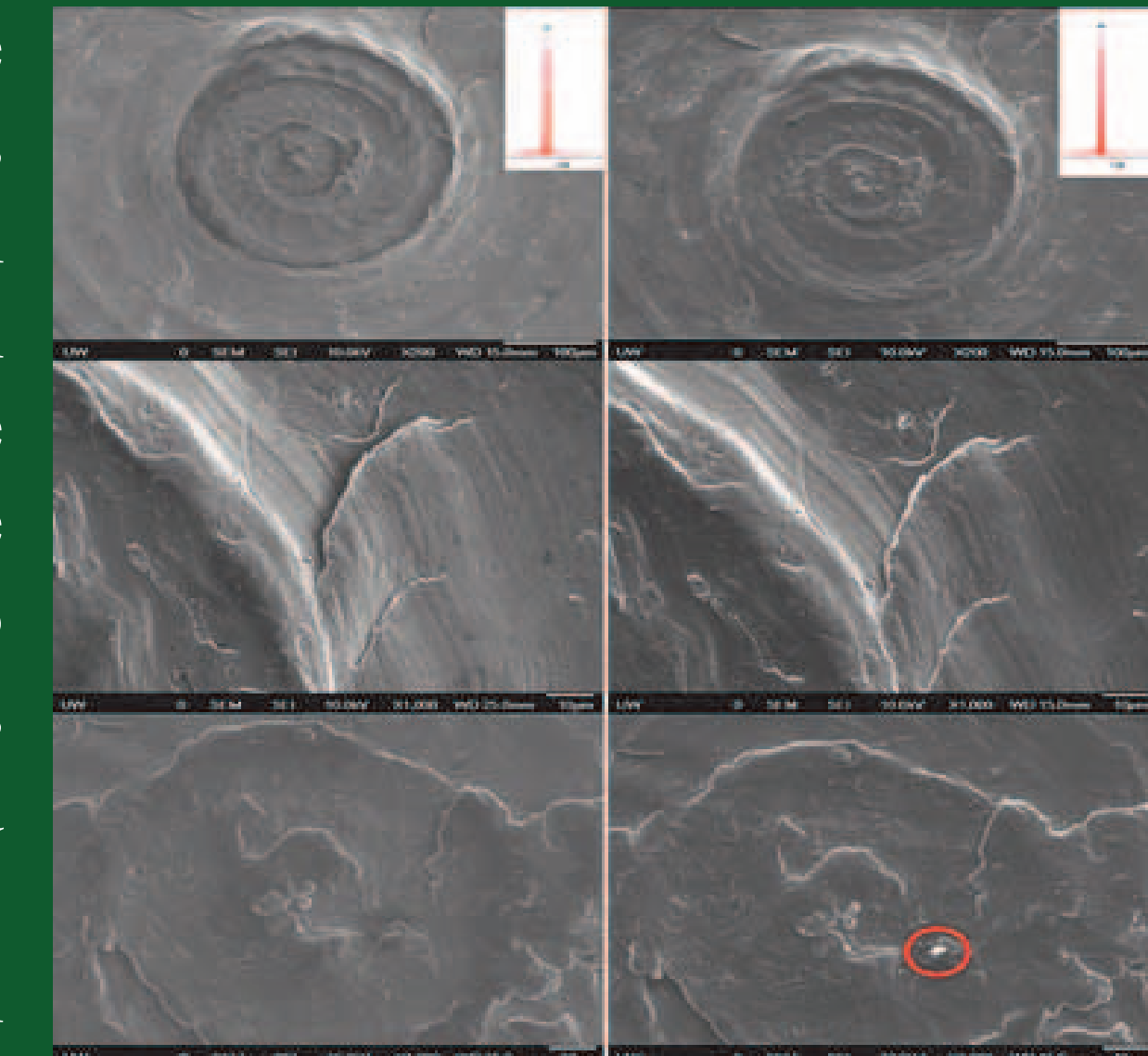
Left Hand Column: SEM images of Al plate before being inserted into plasma. Right Hand Column: SEM images after 300 hydrogen plasma shots (88 ms total exposure time). The red circle indicates the only impurity that could be located.
