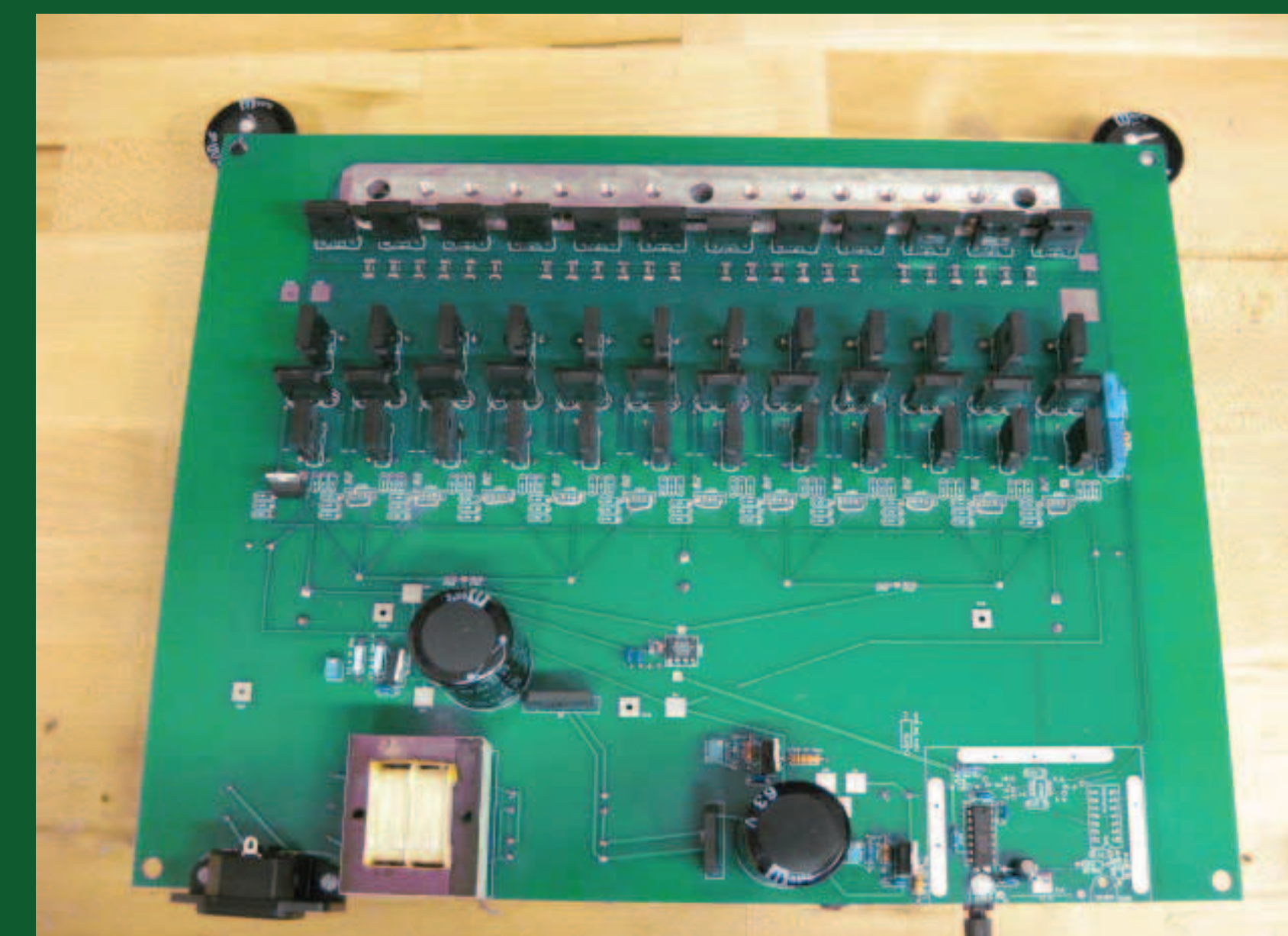
The IGBT switch and snubbers board that formed the basis of the power supply for the EPS antenna system.
