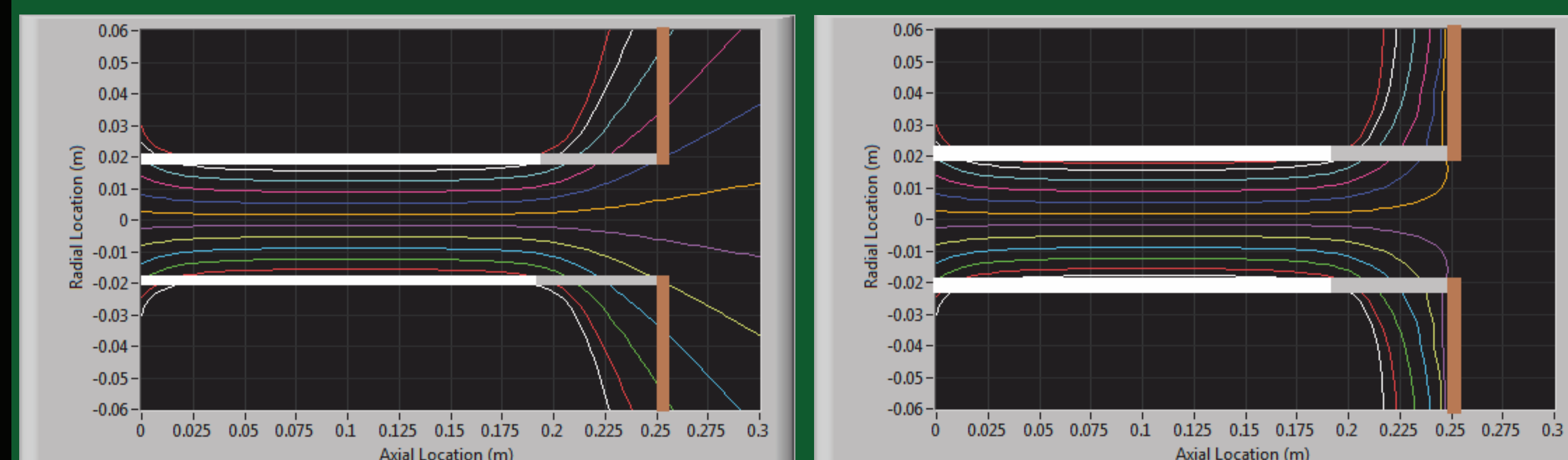
Magnetic field lines during DC (Left) and pulsed operation (Right). White, gray, and tan lines show the approximate vacuum boundaries of various flanges/materials. In both the cases a significant amount of field came into contact with the walls, substantially reducing the maximum amount of plasma that could be injected into the main chamber.
