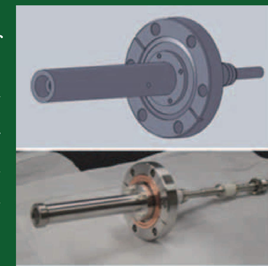
SPG: CAD drawing and completed vacuum hardware.
