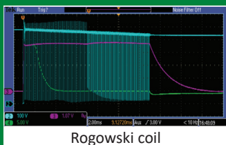
Rogowski coil
